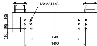
ROBOT TOP VIEW FIXED PLATEN
