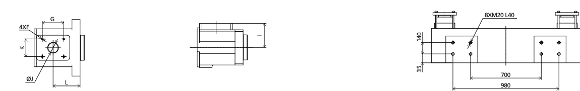
HOPPER MOUNTING DIMENSION
