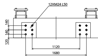
ROBOT TOP VIEW FIXED PLATEN
